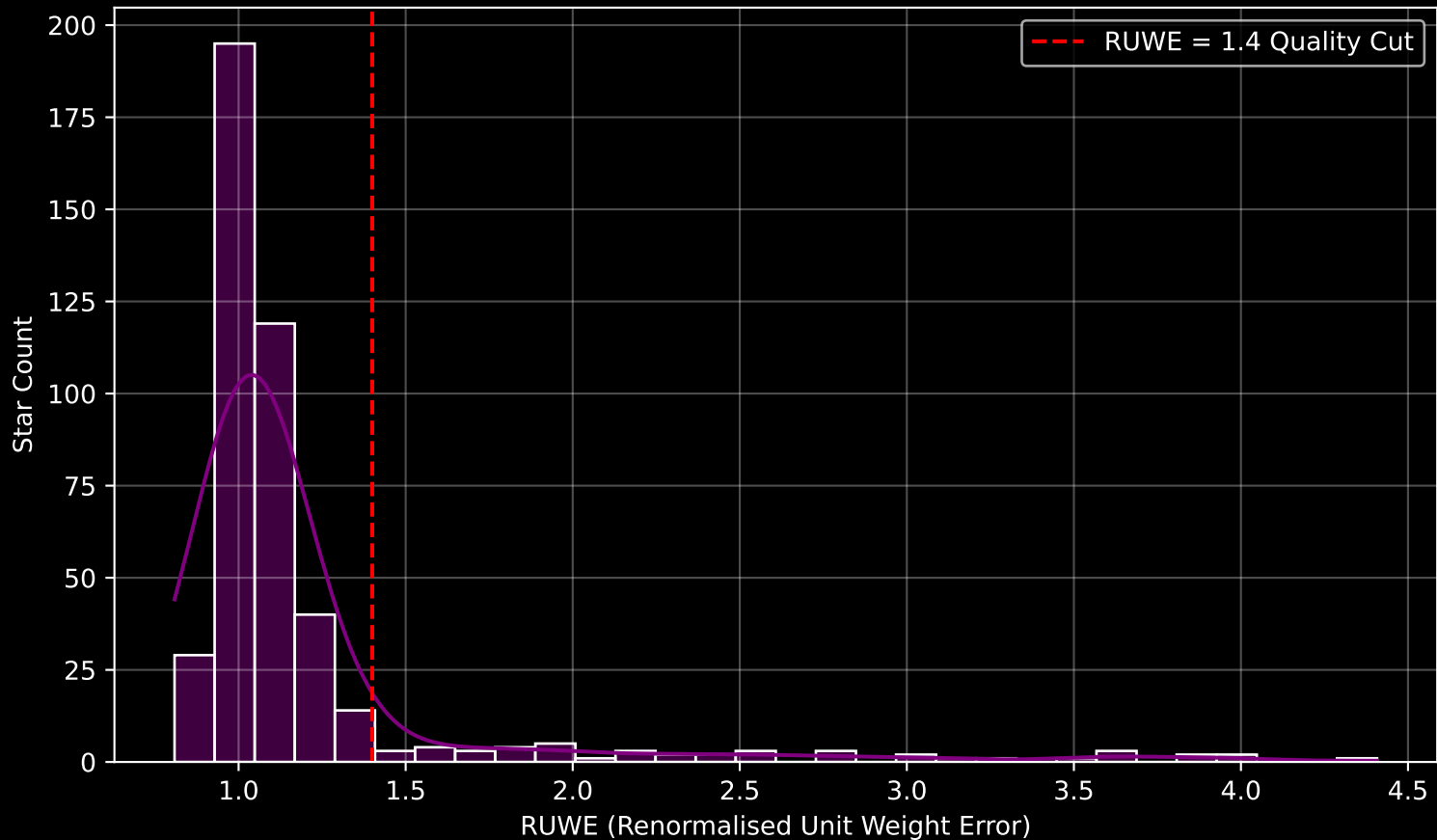
GALAH DR4 Field [6597] RUWE Distribution (n= 443)
