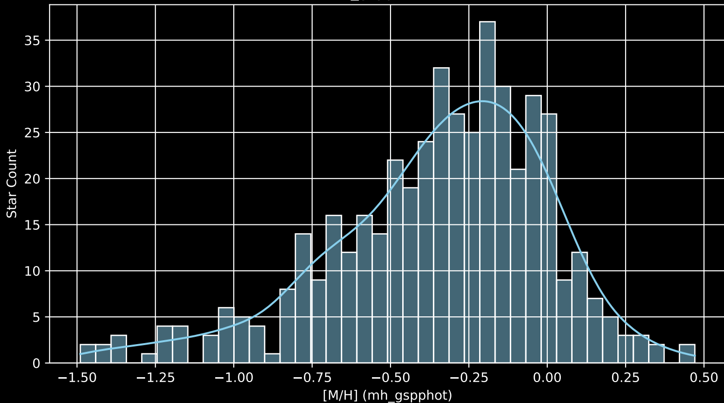
GALAH DR4 Field: [6597] [M/H] (mh_gspphot) (n= 460)
