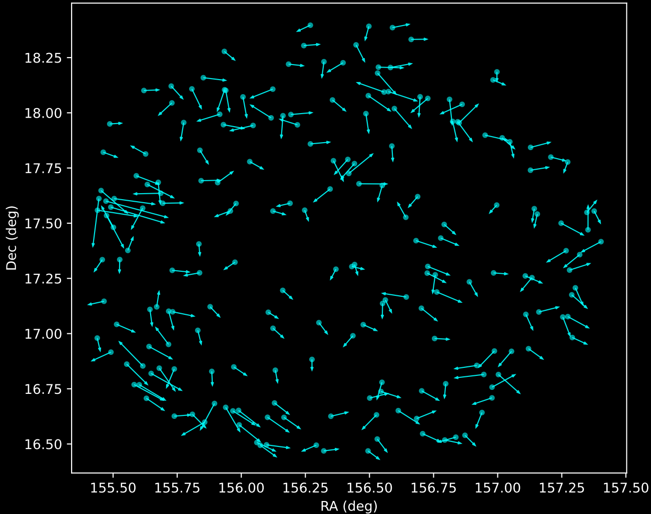
GALAH DR4 Noise Stream Proper Motion Vectors (n=203)
