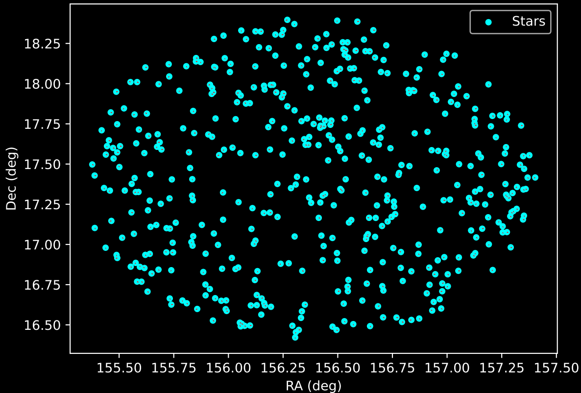
GALAH DR4 Field: [6597] Proper Motion Vectors for Gaia Star Field (n= 462)
