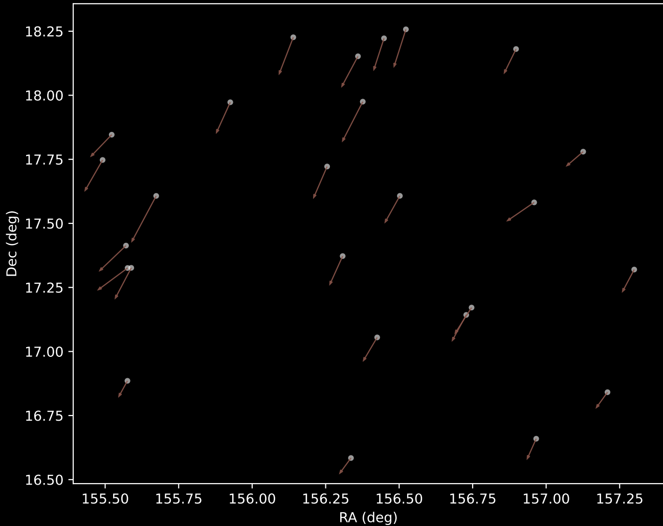
GALAH DR4 Cluster 10 Proper Motion Vectors (n=26)
