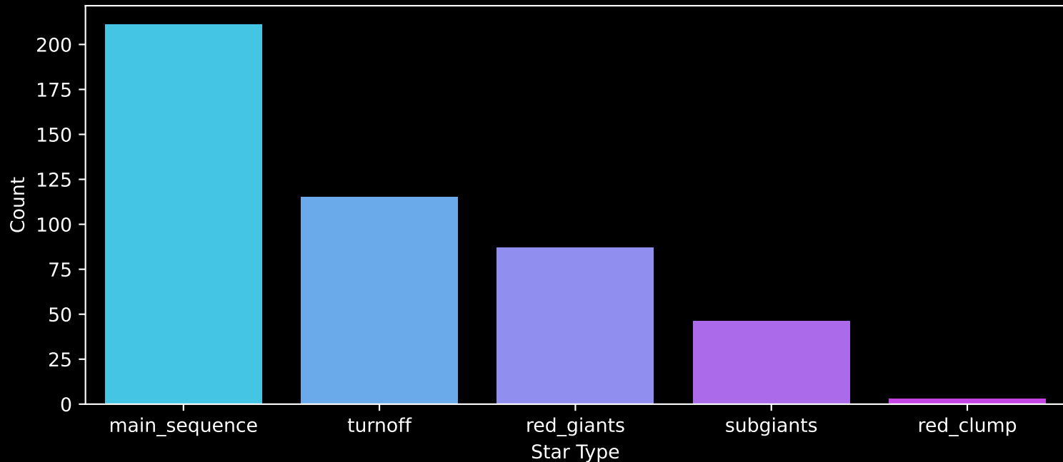
GALAH DR4 Field: [6597] Count plot of Star Type
