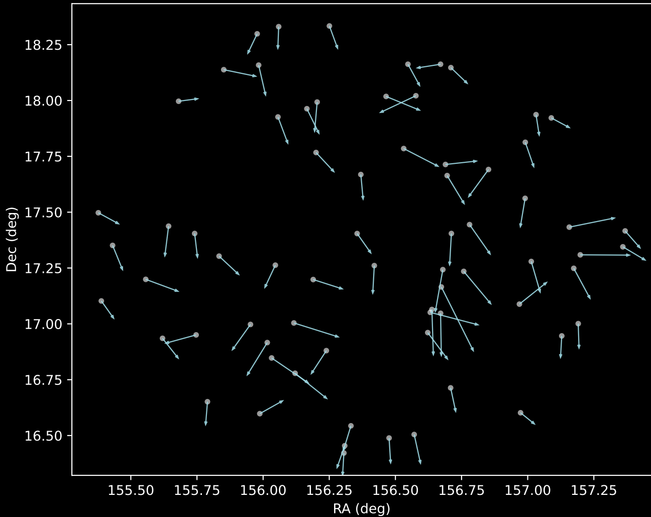
GALAH DR4 Cluster 19 Proper Motion Vectors (n=70)
