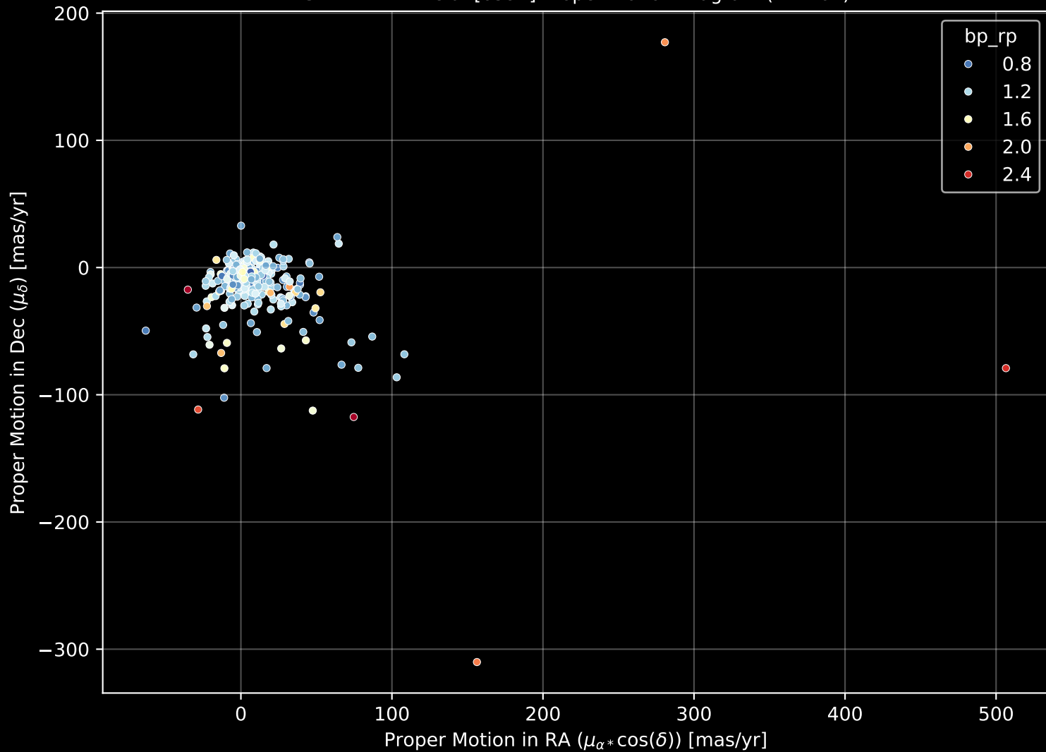
GALAH DR4 Field: [6597] Proper Motion Diagram (n= 462)
